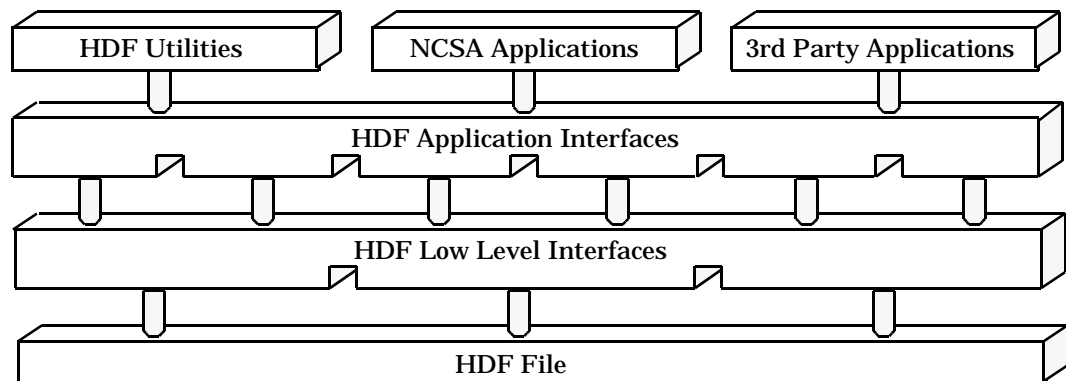
HDF Software Layers
