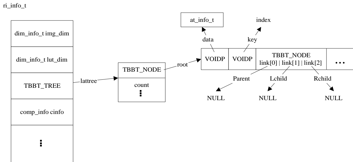
FIGURE 8r Illustration of data structure ri_info_t
