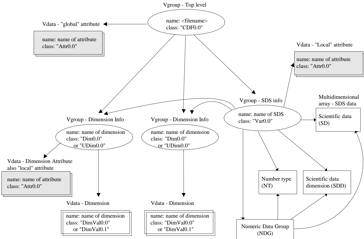
SD collection contents in the file after adding a global attribute, an SDS attribute, and a dimension attribute
