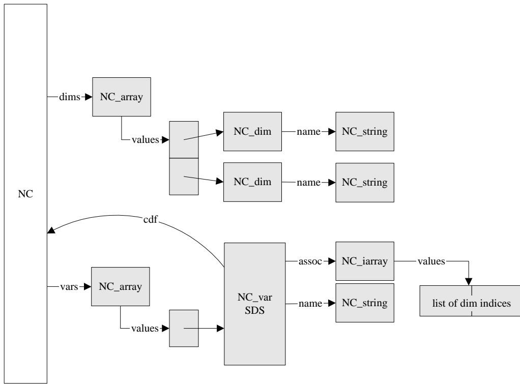
FIGURE 7s SD collection contents in memory after a 2-dimensional SDS is created
