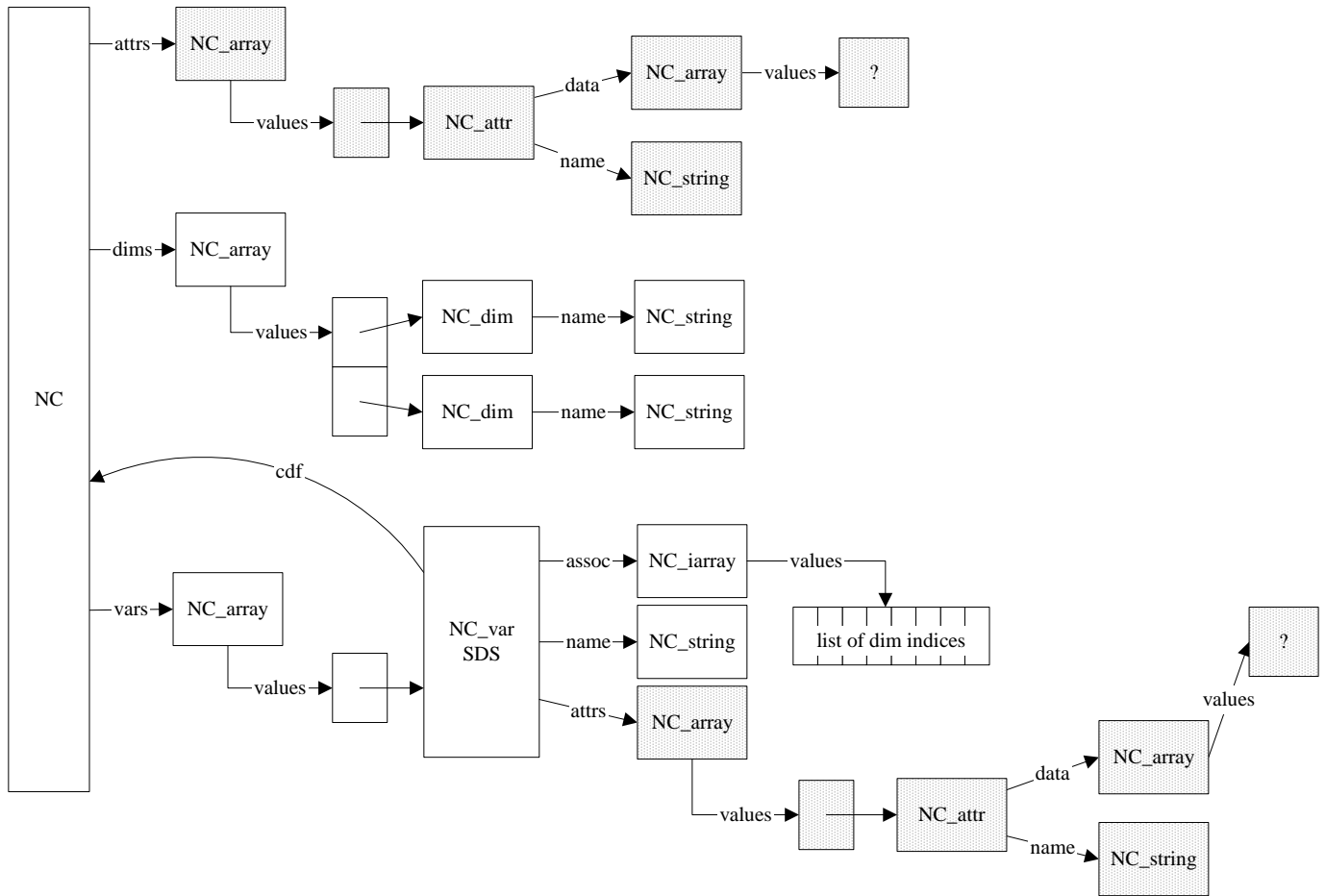
SD collection contents in memory after adding an SDS attribute
