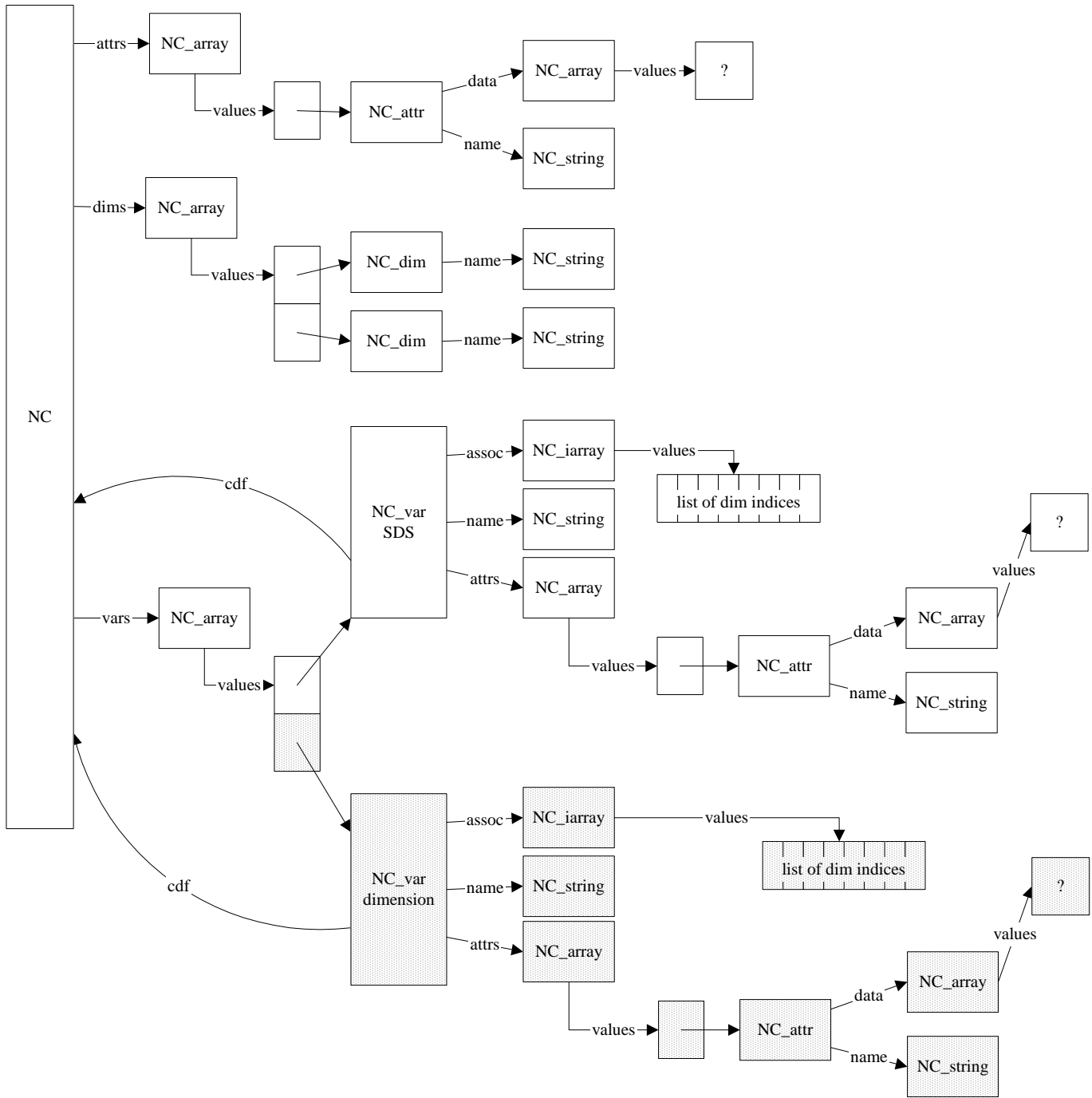
FIGURE 7x SD collection contents in memory after adding a dimension attribute
