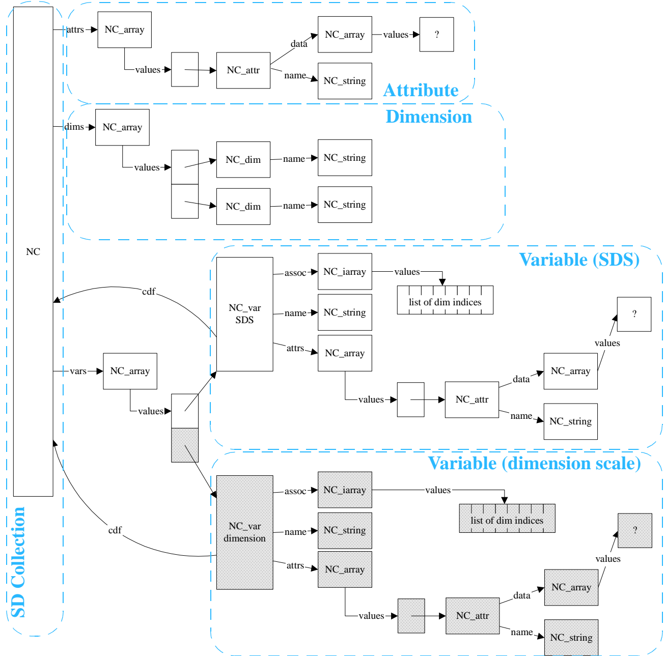
Example of HDF memory structures describing an SD collection
