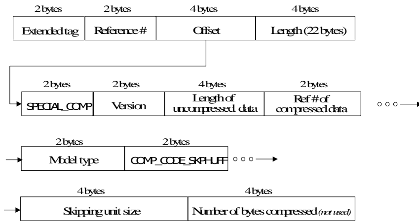
Extended tag description for Skipping-Huffman compression
