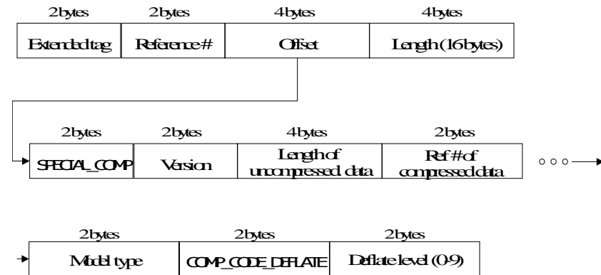
Extended tag description for GNU ZIP (deflate) compression
