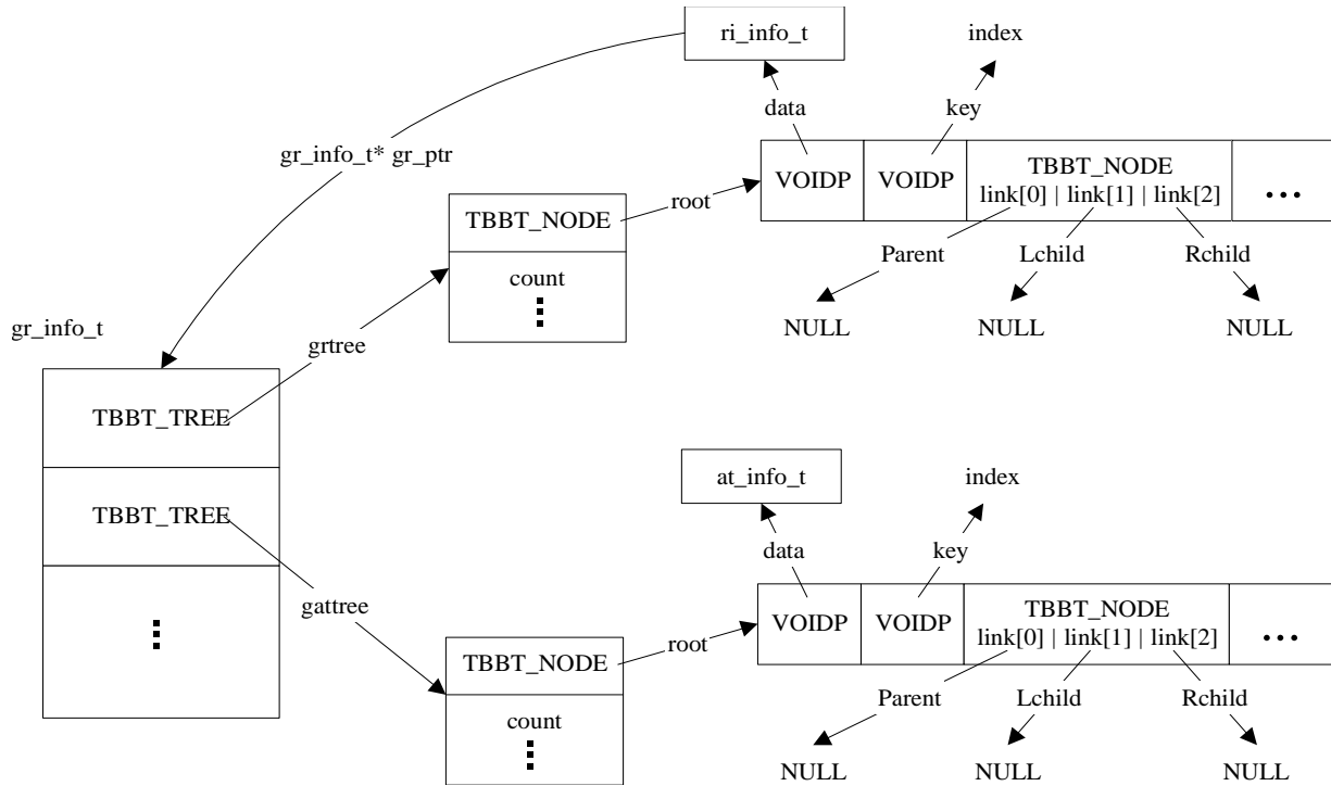
FIGURE 8q Illustration of data structure gr_info_t
